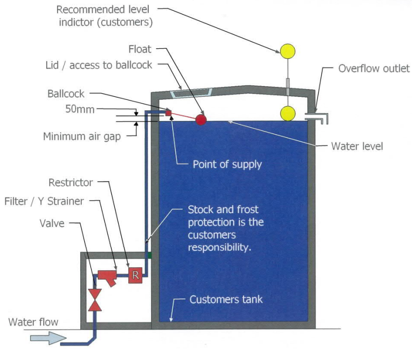
Standard pipework
