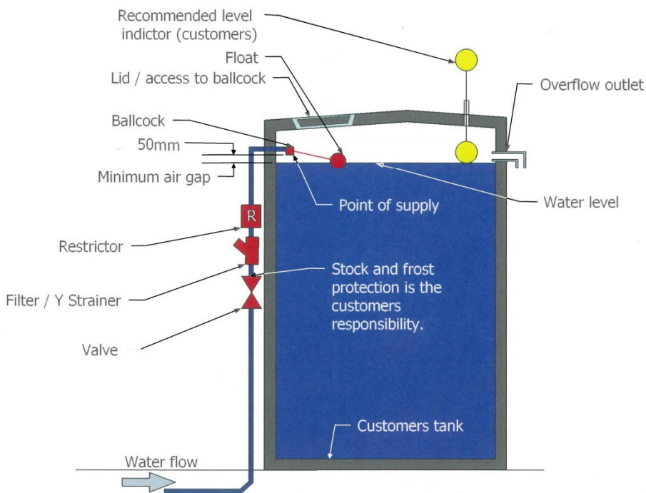
Alternative pipework
